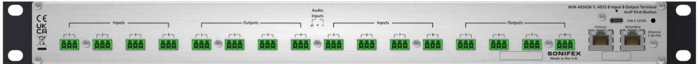
Fig 2-3: AVN-AESIO8-T-DNT Rear Panel
