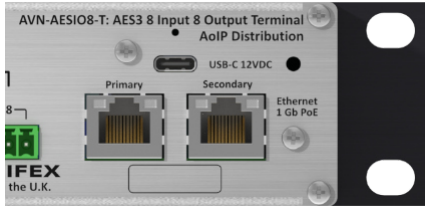
Fig 2-6: Ethernet, PoE & USB-C Connections
