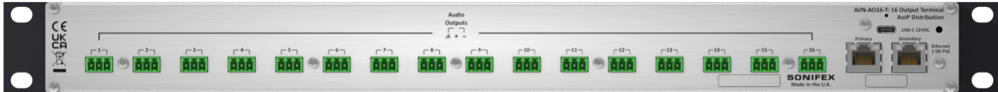
Fig 2-5: AVN-AO16-T-DNT Rear Panel
