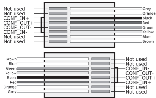
Figure 3-2: Conference Port Cable Connections.
