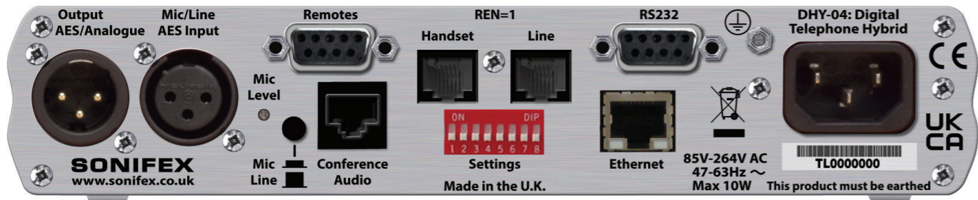
Figure 1-1: DHY-04 Front & Rear.
