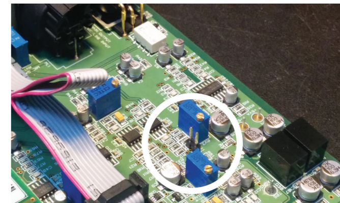
Figure 2-2: Internal Position of Jumper J1.
