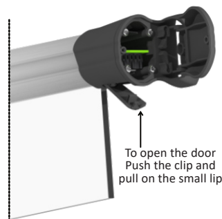
Fig 2-5: Opening The Access Door
