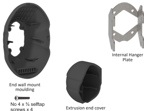
Fig 5-2: Kit Components Used for the Conversion
