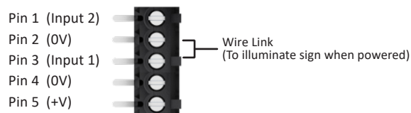
Fig 2-9: Wire link To Illuminate Sign When Powered
