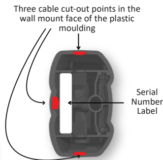
Fig 2-4: Cable Routing Cut-Outs
