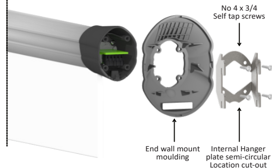
Fig 5-3: Removing the Left Hand Assembly
